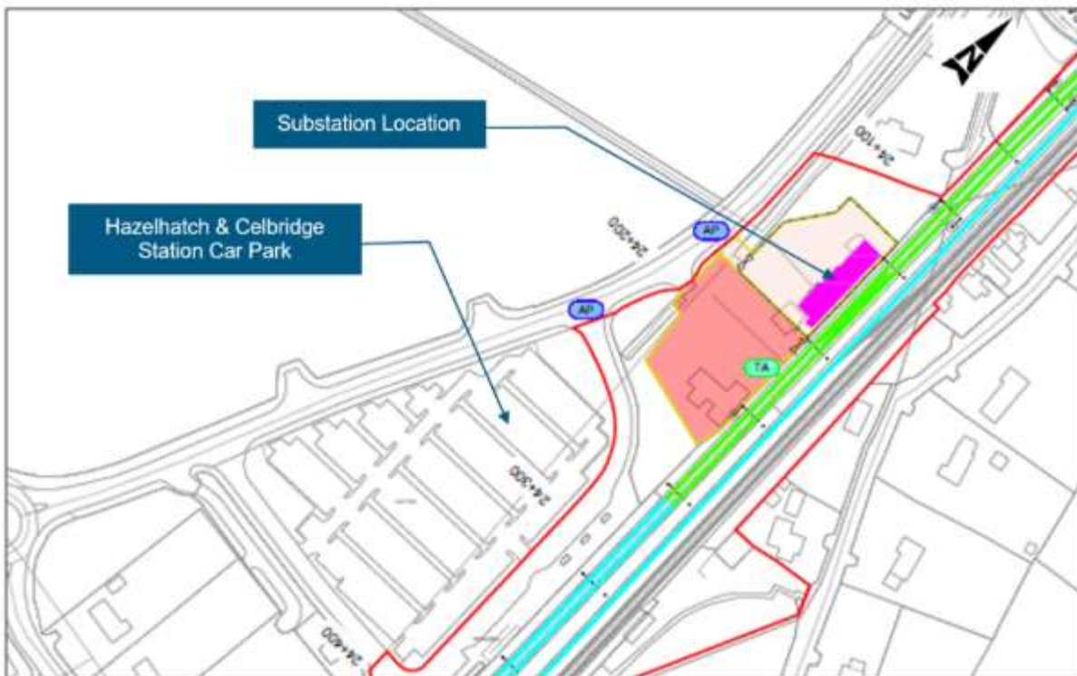
Figure 5-22 Indicative Hazelhatch Substation Layout
